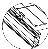
middle clamp
